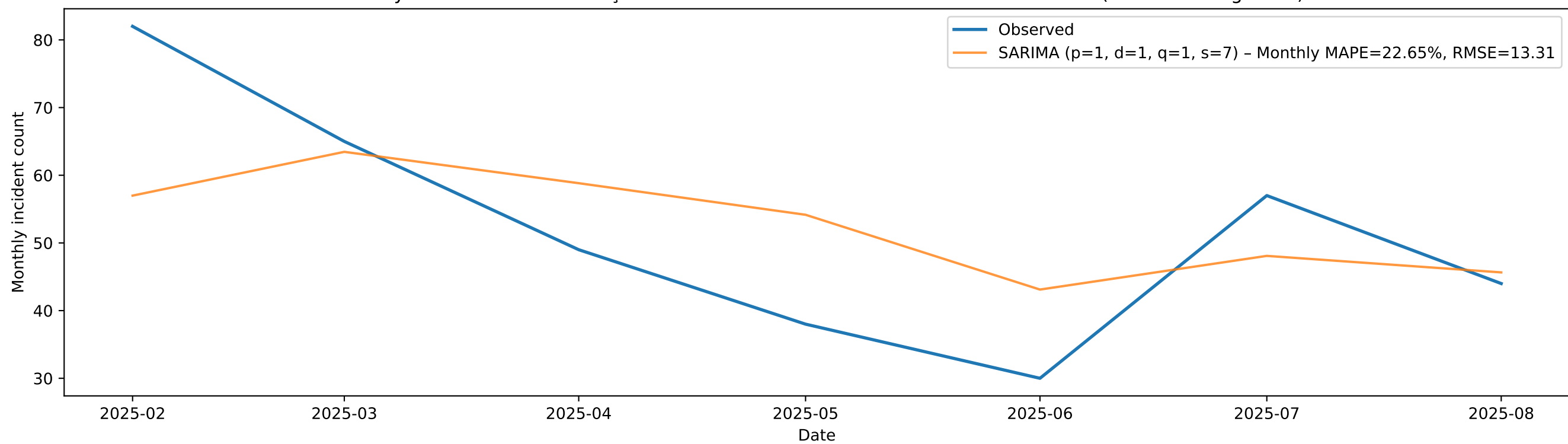
Monthly Traffic Incidents in Yeşildere Street: Best Time-series Model vs Observed (Feb 2025-Aug 2025)
